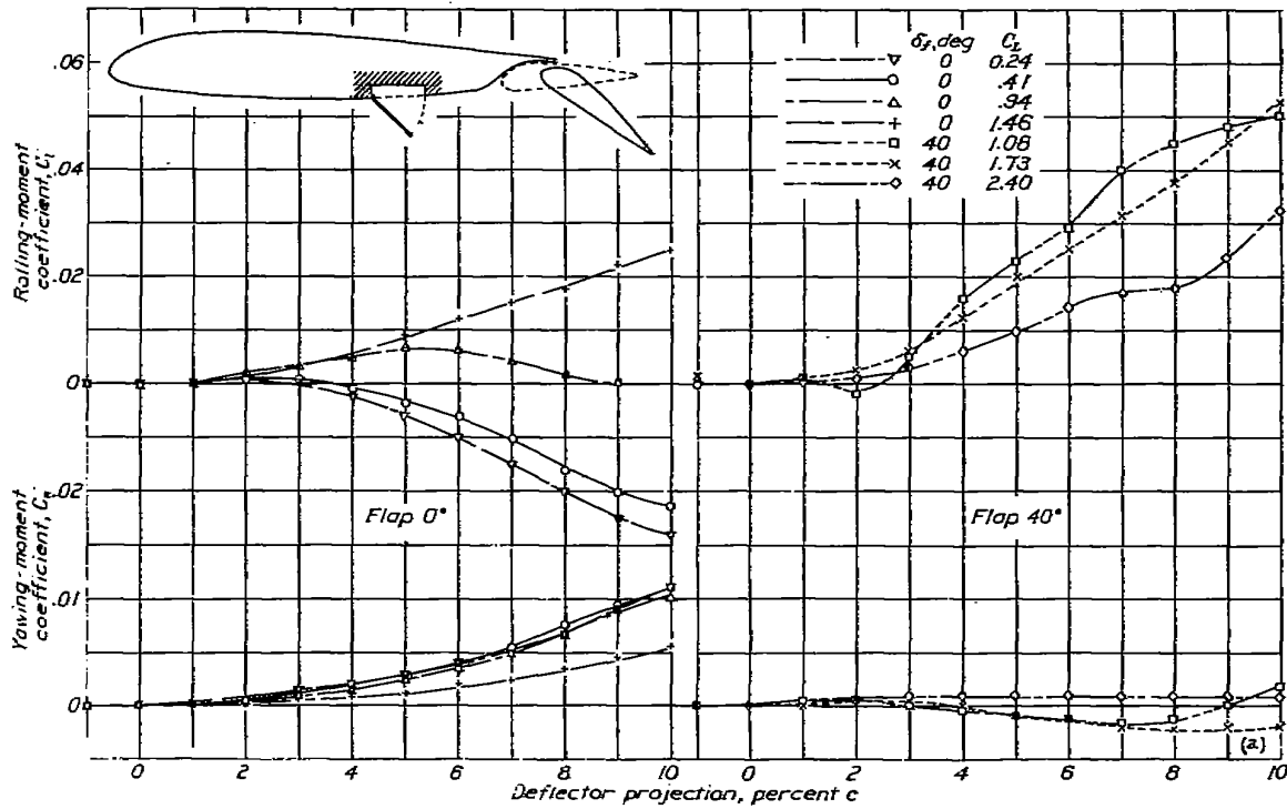
(a) Rolling- and yawing-moment coefficients.
