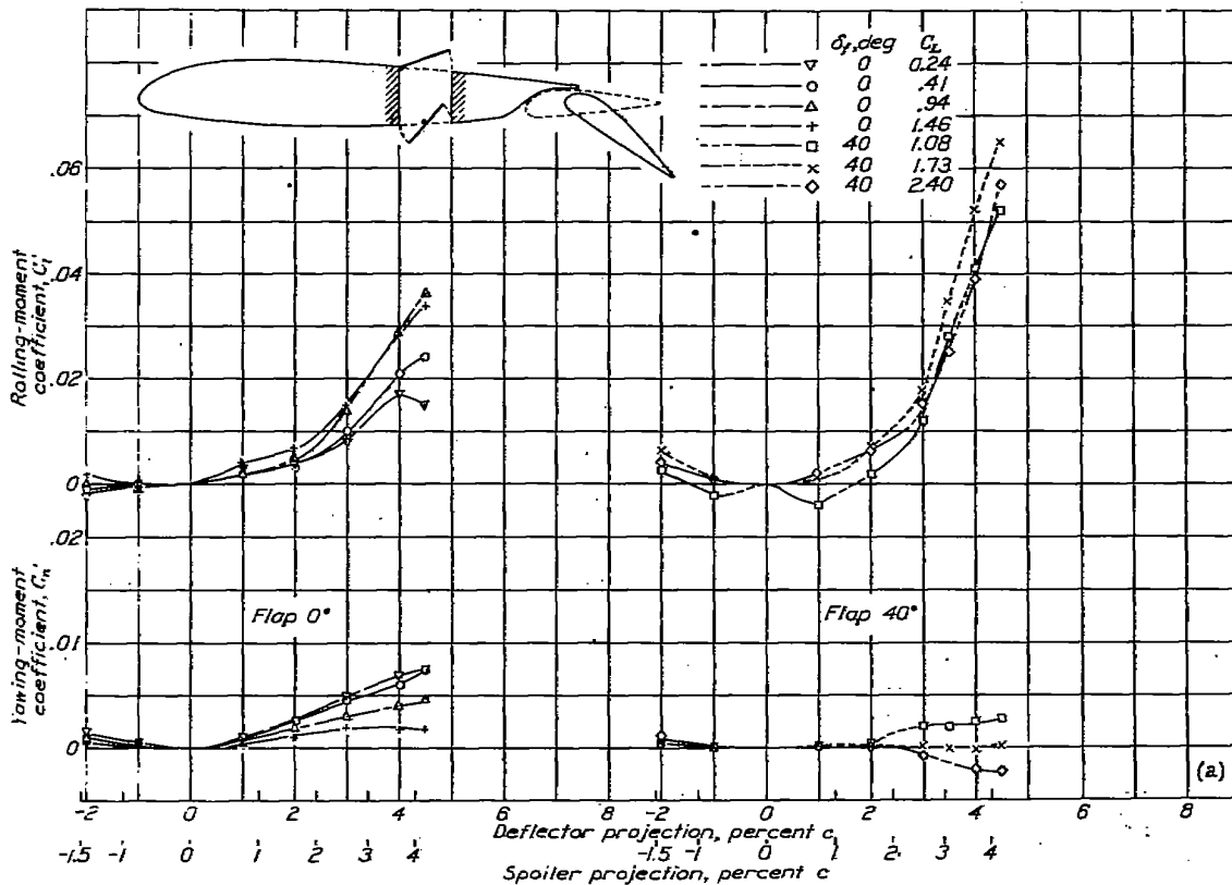
(a) Rolling- and yawing-moment coefficients.
