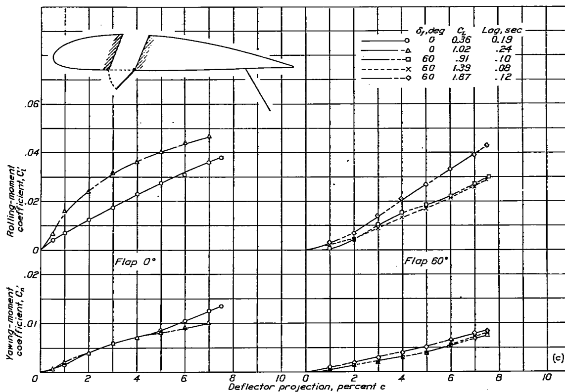
FIGURE 22.—Rolling- and yawing-moment coefficients due to an 0.11c deflector hinged at 0.31c and a slot on a Clark Y-15 wing with a 0.20c full-span split flap
