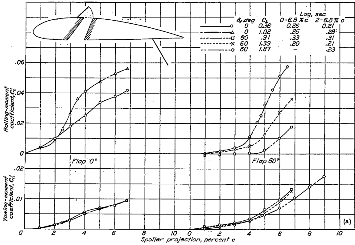
(a) Spoiler hinge at 0.20c.
