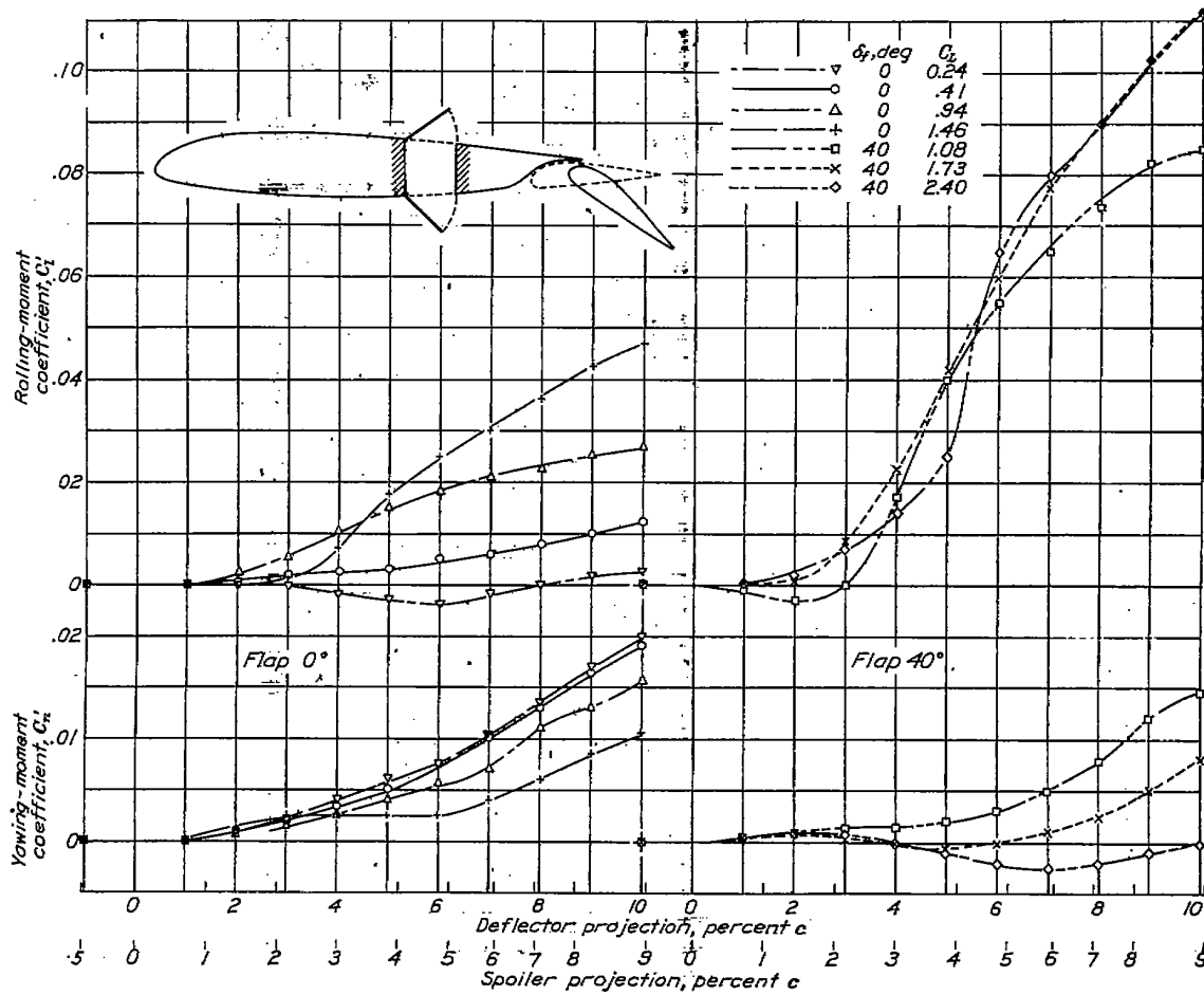
FIGURE 19.—Rolling- and yawing-moment coefficients due to a 0.10c spoiler hinged at 0.50c and a 0.10c deflector hinged at 0.50c with a slot on an NACA 23012 wing with a 0.250c full-span slotted flap.
