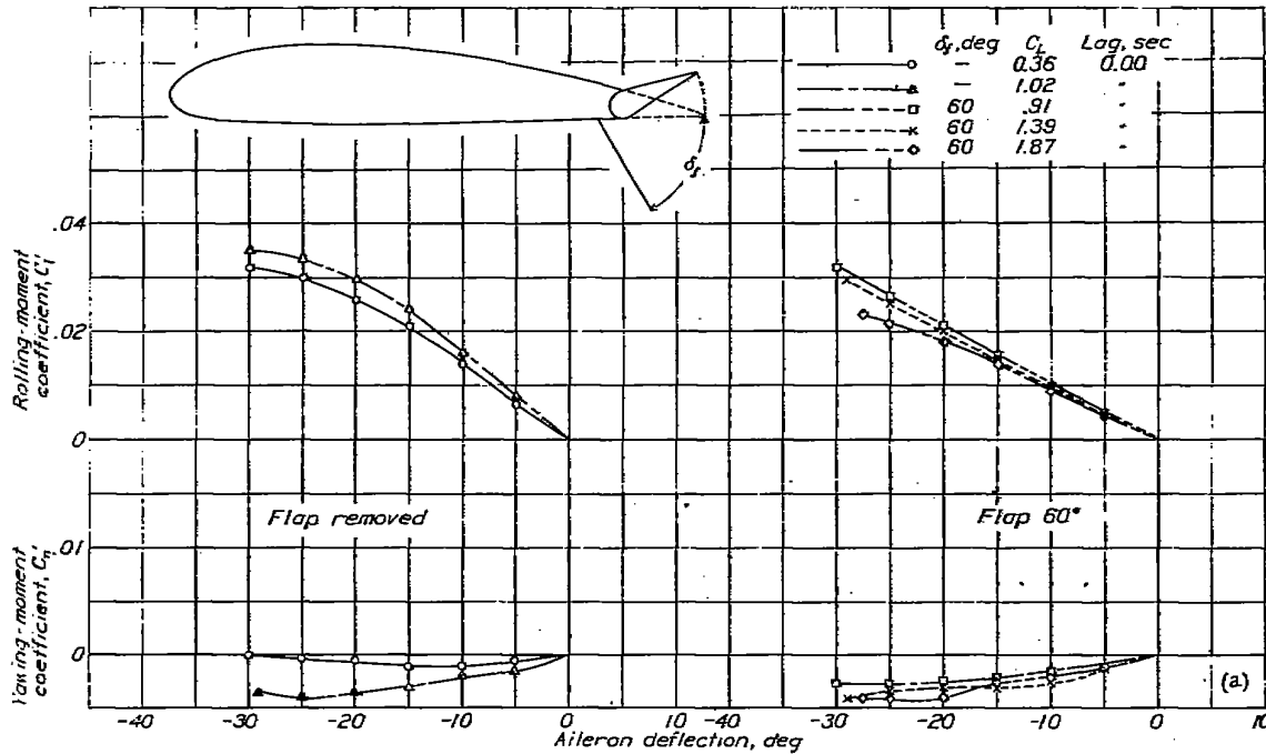
(a) Rolling- and yawing-moment coefficients.
