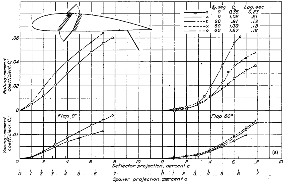
(a) Spoiler hinge at 0.23c; deflector hinge at 0.34c; slot width at top, 0.06c.
