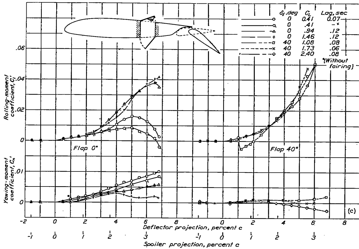
(c) Projection ratio of spoiler to deflector, 1:2.
