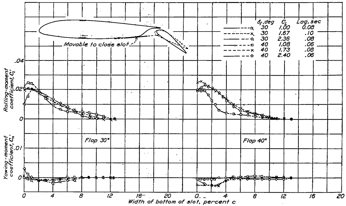
FIGURE 11.—Rolling- and yawing-moment coefficients due to a slot-closing deflector on an NACA 23012 wing with a 0.2568c full-span slotted flap.
