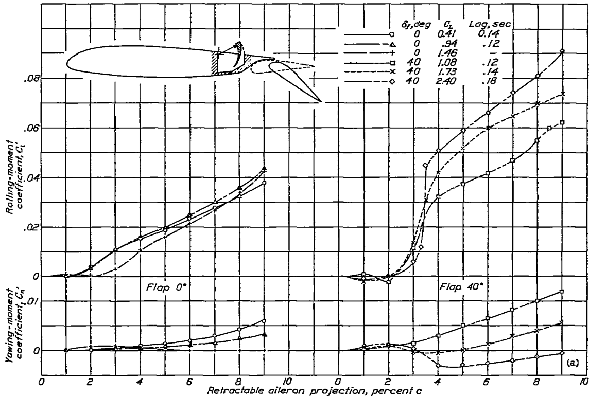
(a) Rolling- and yawing-moment coefficients.
