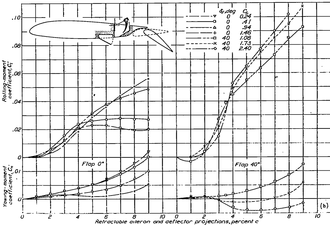
(b) Projection ratio of aileron to deflector, 1:1.
