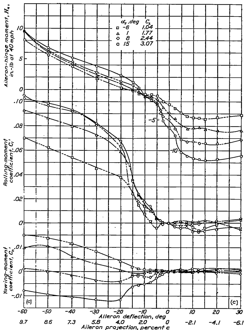
(c) The 0.2586c slotted flap deflected 40°.
