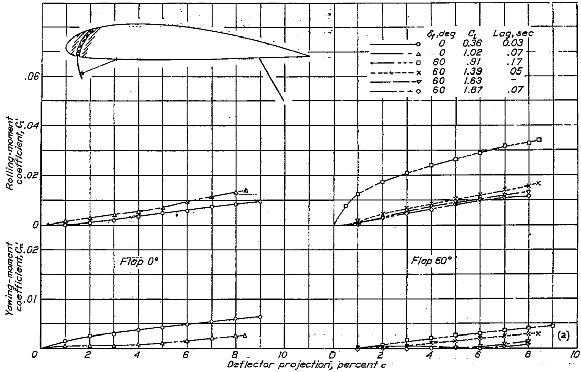
(a) Retractable deflector at 0.05c.
