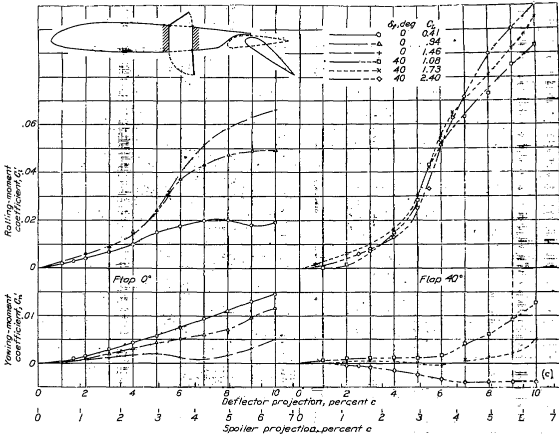
(c) Spoiler hinge at 0.50c; deflector hinge at 0.60c; projection ratio of spoiler to deflector about 2:3.
