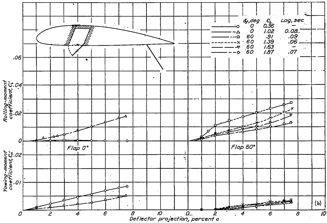
(b) An 0.11c deflector hinged at 0.34c.
