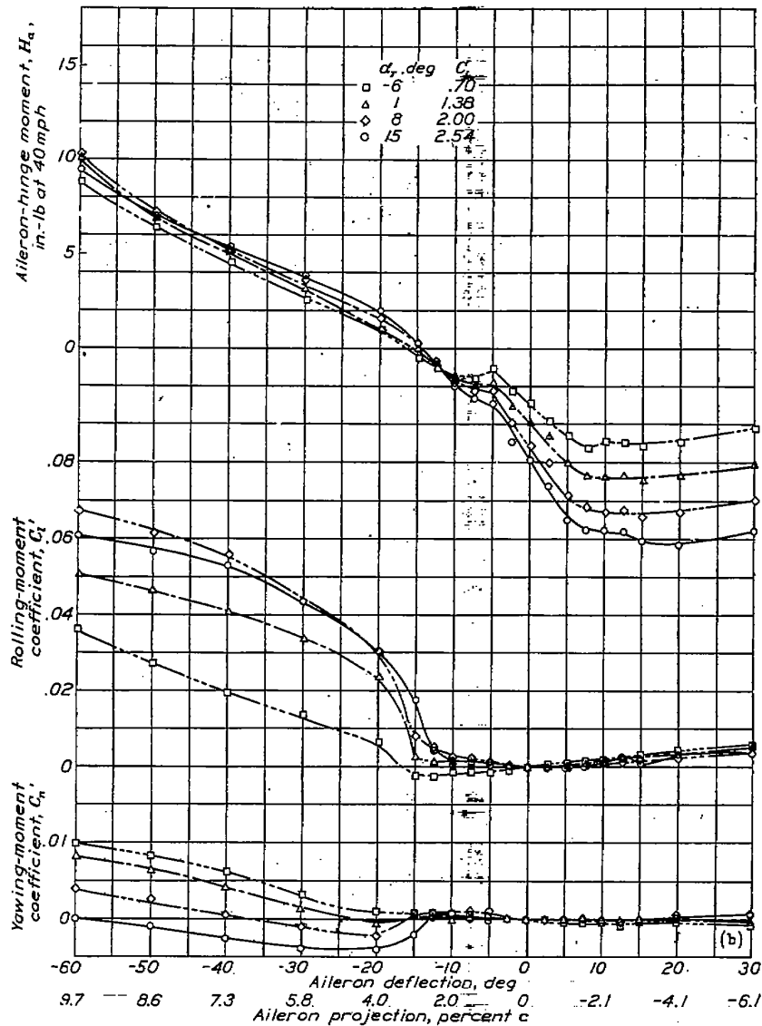
(b) The 0.20c split flap deflected 60°.
