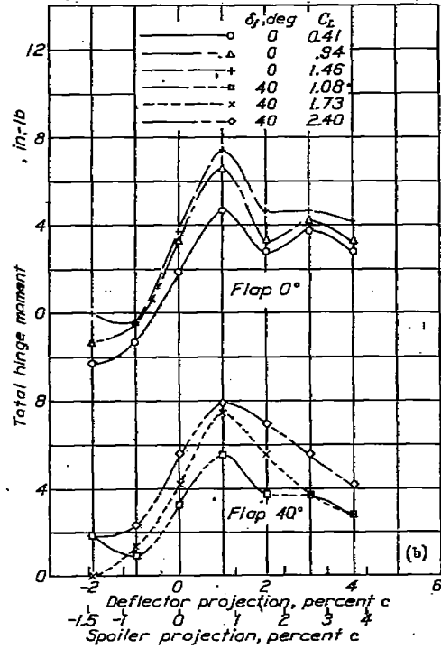
(b) Hinge moment, measured at deflector, at 40 miles per hour. FIGURE 21.—A 0.10c spoiler hinged at 0.50c and a 0.10c deflector hinged at 0.55c with a slot on an NACA 23012 wing with a 0.2566c full-span slotted flap.
