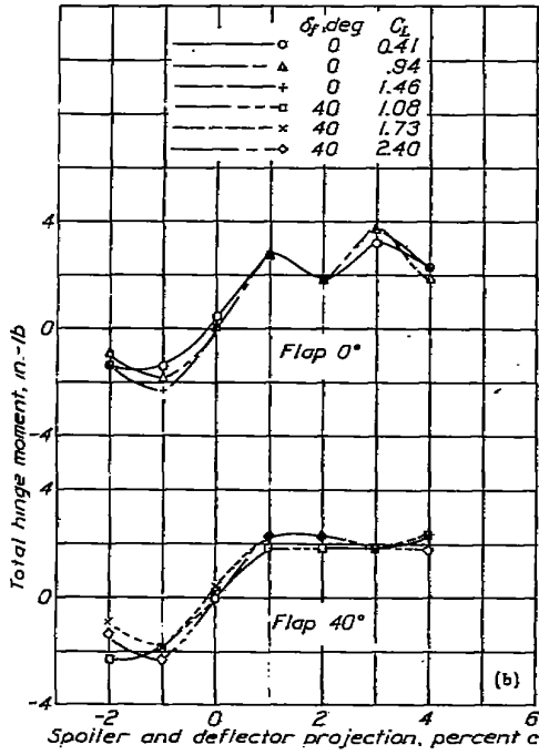
(b) Hinge moment at 40 miles per hour. FIGURE 20.—A 0.10c spoiler hinged at 0.55c and a 0.10c deflector hinged at 0.55c with a slot on an NACA 23012 wing with a 0.2566c full-span slotted flap.
