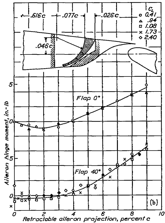
(b) Hinge moment at 40 miles per hour. FIGURE 7.—A retractable aileron on an NACA 23012 wing with a 0.2566c full-span slotted flap.
