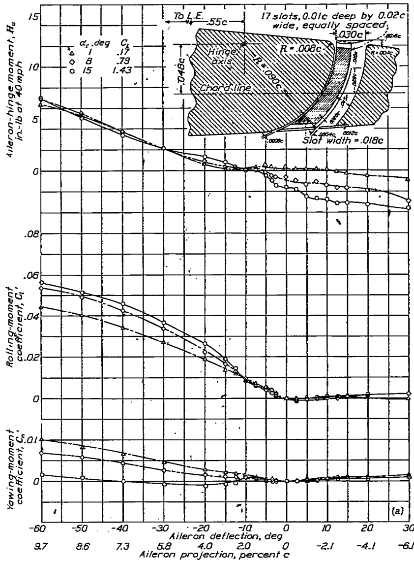
(a) Flap neutral. FIGURE 24.
