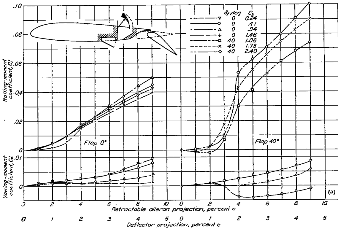
(a) Projection ratio of aileron to deflector, 2:1.
