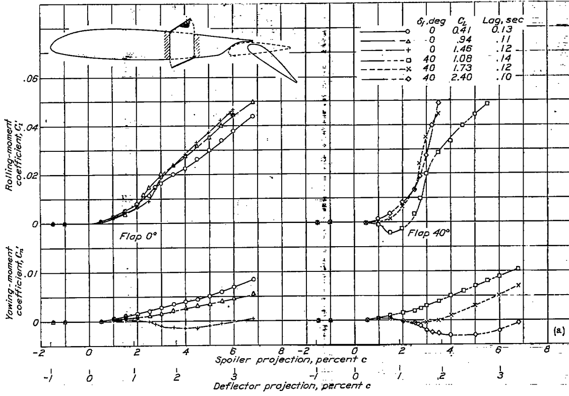
(a) Projection ratio of spoiler to deflector, 2:1.
