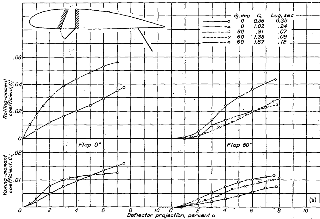
(b) Slot width at top, 0.05c.
