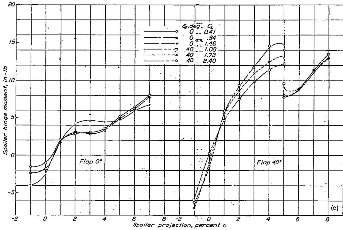
(c) Hinge moment at 40 miles per hour; spoiler hinge at 0.60c . FIGURE 5.—A 0.10c spoiler on an NACA 23012 wing with a 0.266c full-span slotted flap.
