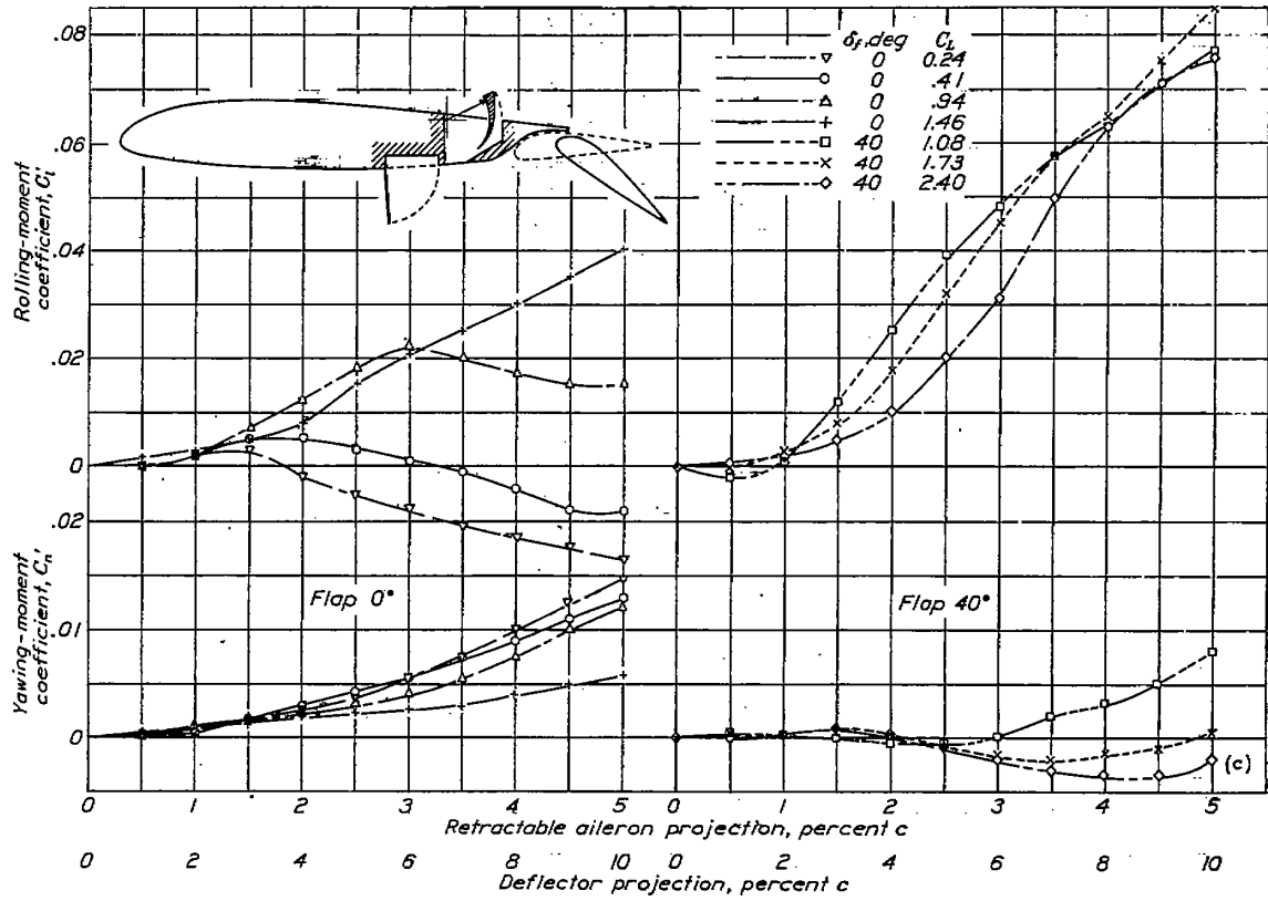
(c) Projection ratio of aileron to deflector, 1:2.
