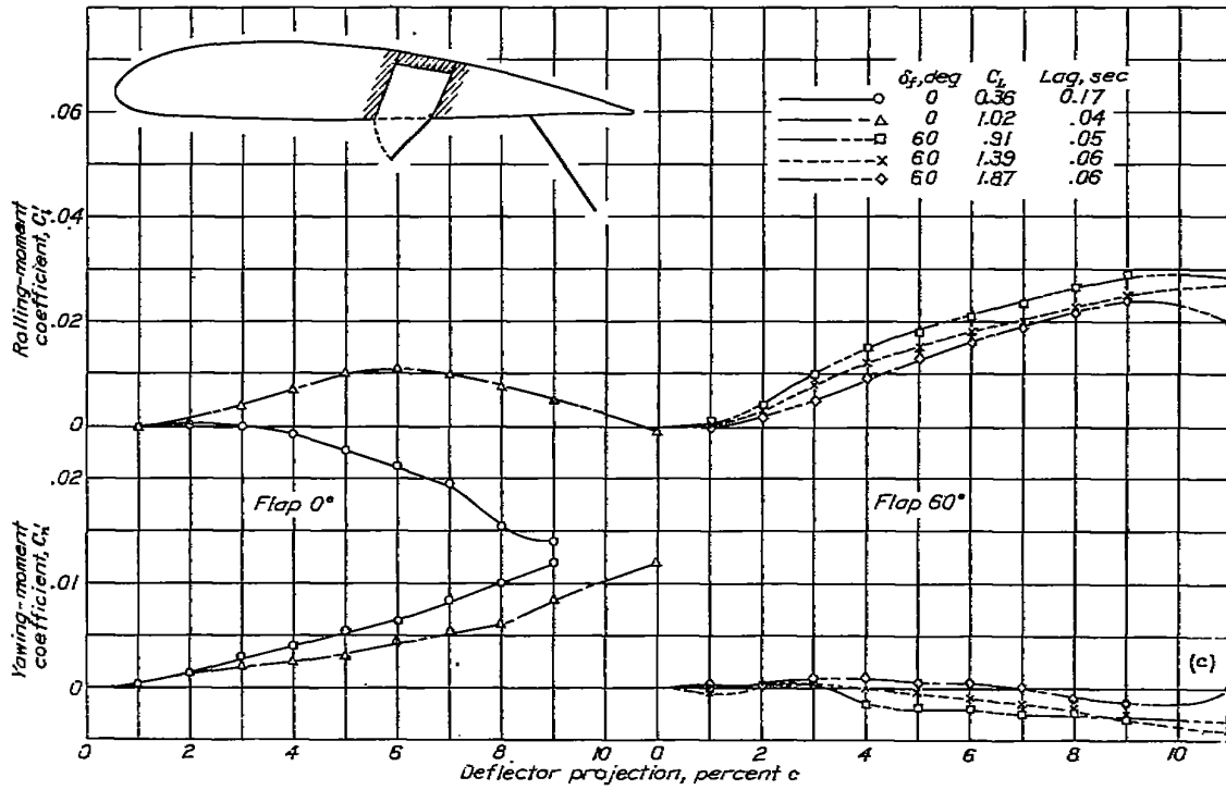
(c) An 0.11c deflector hinged at 0.61c.
