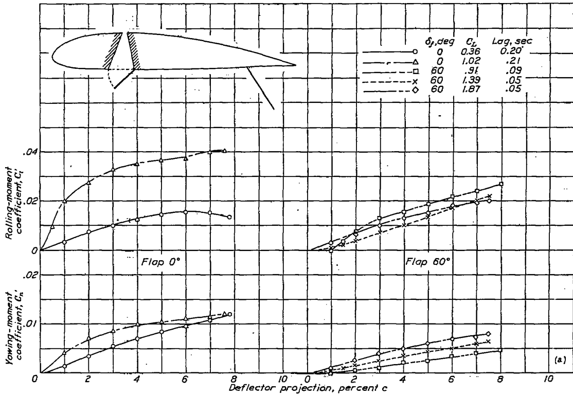
(a) Slot width at top, 0.02c.
