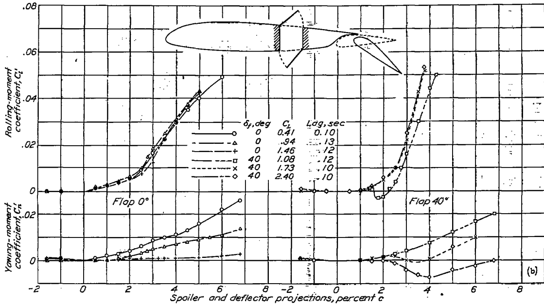
(b) Spoiler hinge at 0.50c; deflector hinge at 0.60c; projection ratio of spoiler to deflector, 1:1.
