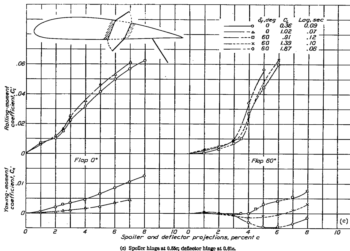
FIGURE 15.—Rolling- and yawing-moment coefficients due to an 0.11c spoiler and an 0.11c deflector with a slot on a Clark Y-15 wing with a 0.20c full-span split flap.
