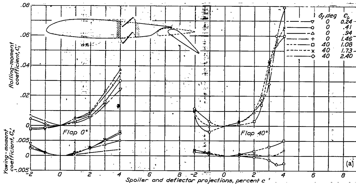
(a) Rolling- and yawing-moment coefficients.
