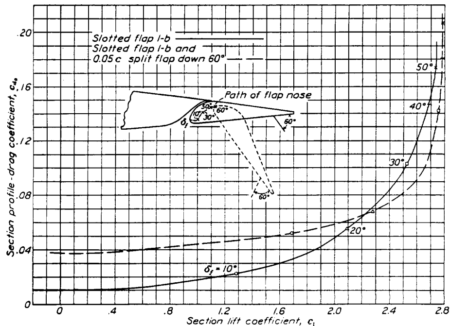
FIGURE 28.—Effect on c_{p_0} of combining split flap with slotted flap. Slotted flap 1-b.
