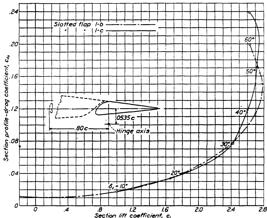
FIGURE 13.—Comparison of slotted flaps 1-a and 1-b.
