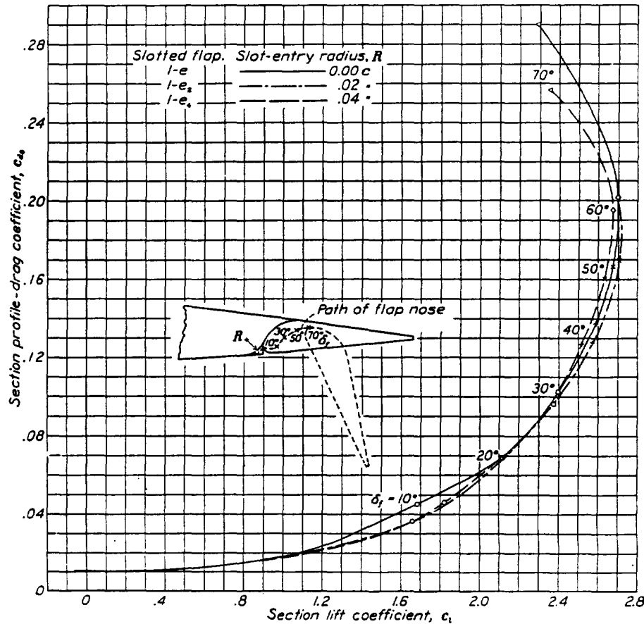
FIGURE 24.—Effect of slot-entry radius on c_{d_0} .
