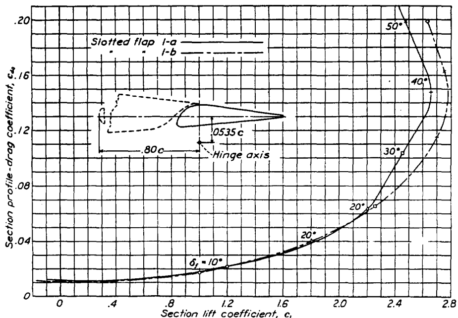
FIGURE 14.—Comparison of slotted flaps 1-b and 1-c.
