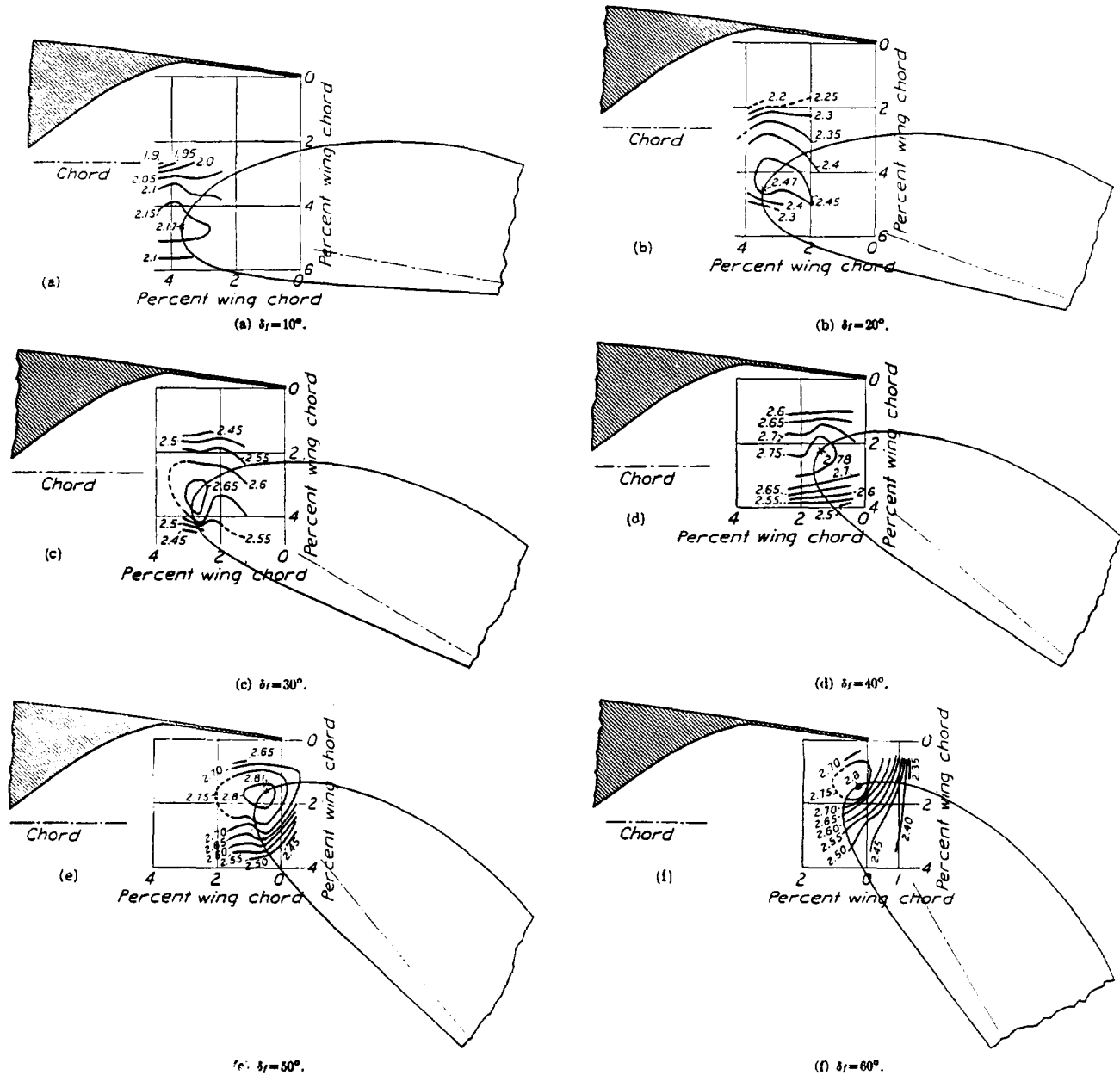
FIGURE 18.—Contours of flap location for c_{max} . Slotted flap 2-h.
