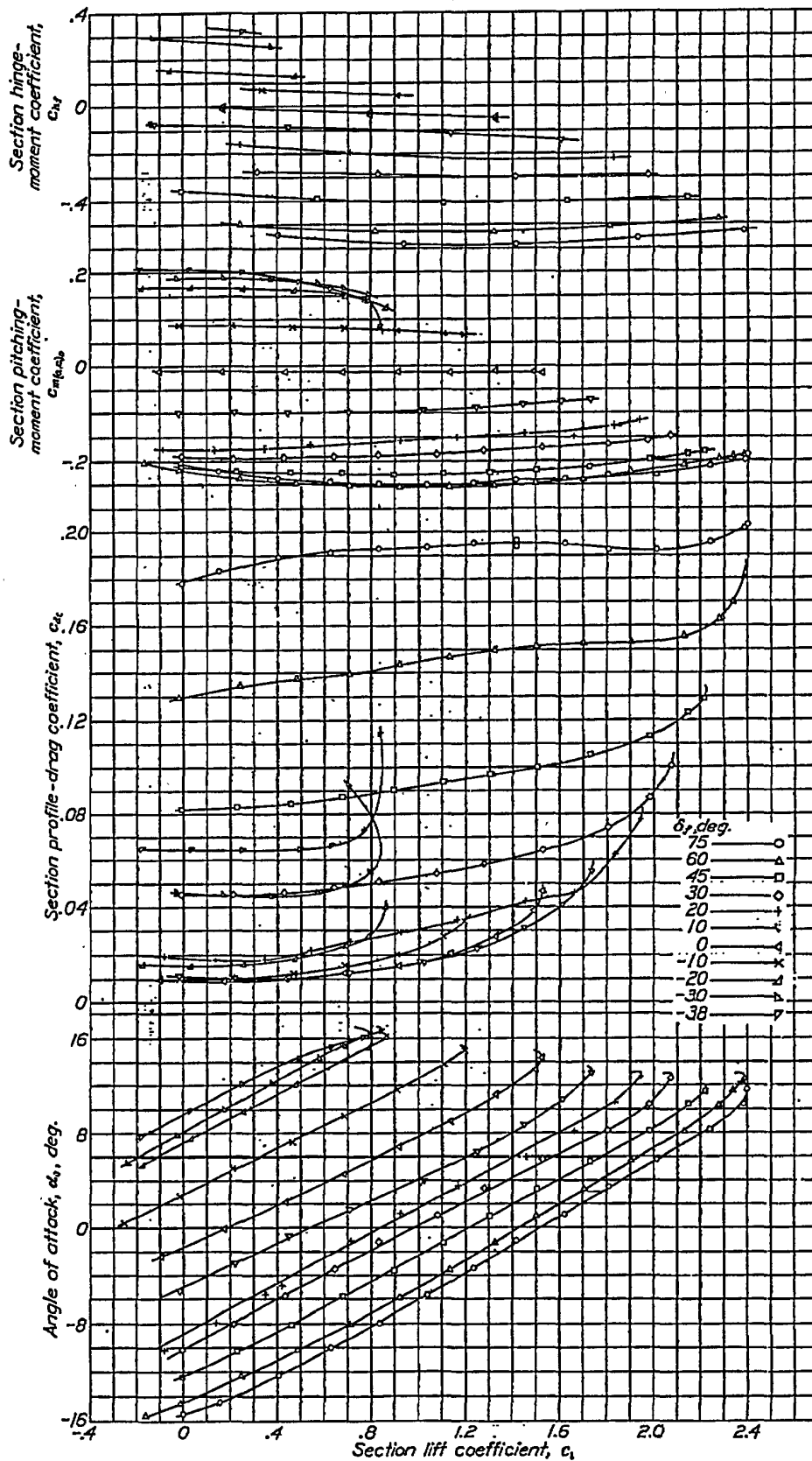
FIGURE 2.—Section aerodynamic characteristics of N. A. C. A. 23012 airfoil with a 0.20c plain flap.
