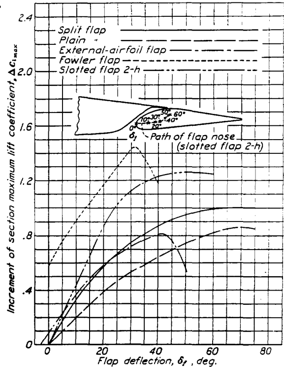
FIGURE 30.—Comparison of increments of maximum lift coefficients for five types of flap.
