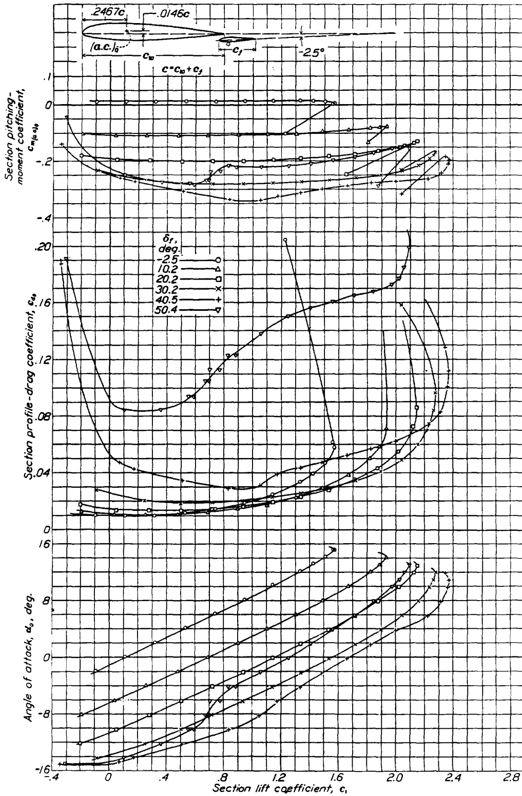
FIGURE 10.—Section aerodynamic characteristics of N. A. C. A. 23012 airfoil with a 0.2667c w N. A. C. A. 23012 external-airfoil flap.
