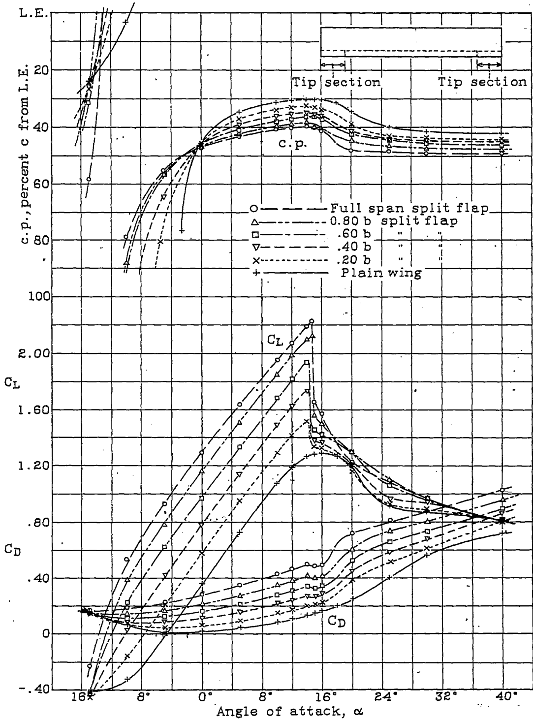
Figure 3.- Split flaps with tip sections removed
