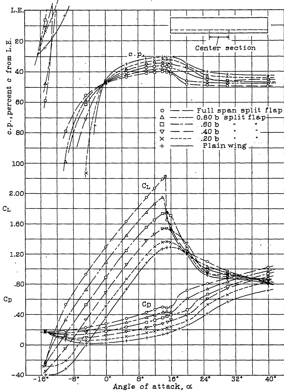
Figure 4. - Split flaps with center sections removed
